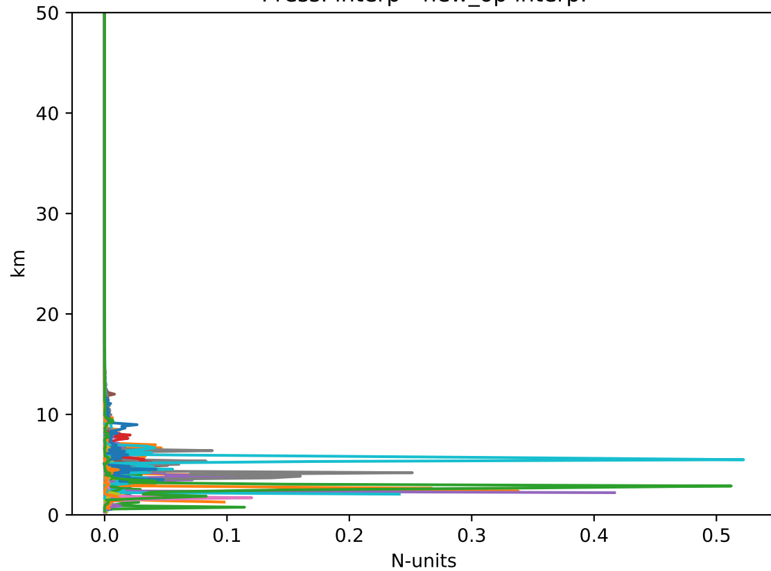
Figure 1, background refractivity interpolation biases, ERA5 (27 profiles)
